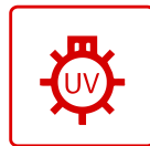
Polymerization
